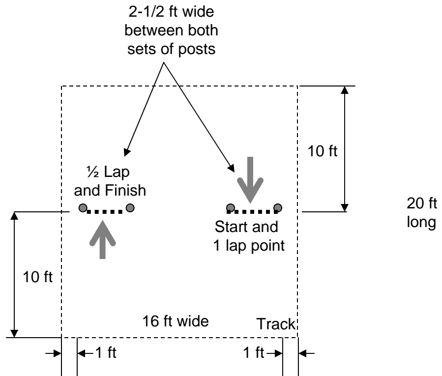
Layout and dimensions of a track.
